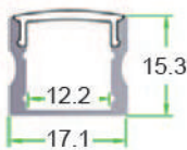
Dimensions in mm
